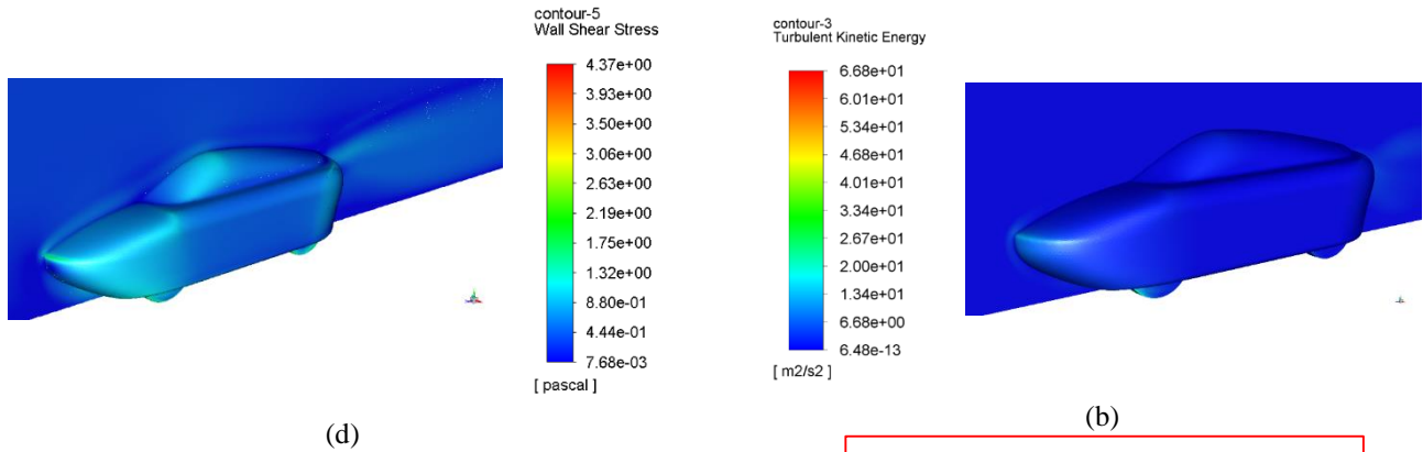
Figure 8. (a) Pressure, (b) Turbulent Kinetic Energy , (c) Velocity Magnitude, and (d) Wall Shear Stress figures at 16.67 m/s
