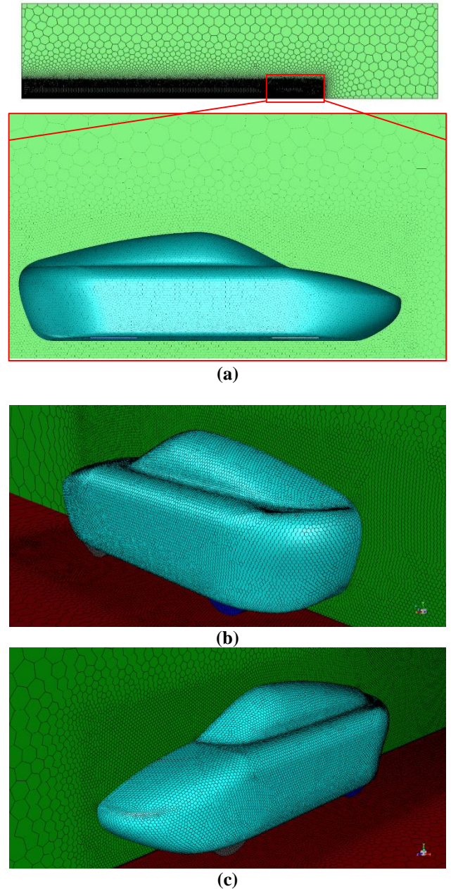
Figure 3. (a) Detailed view (b) Rear Isometric view (c) Front Isometric view of polyhedral meshing
