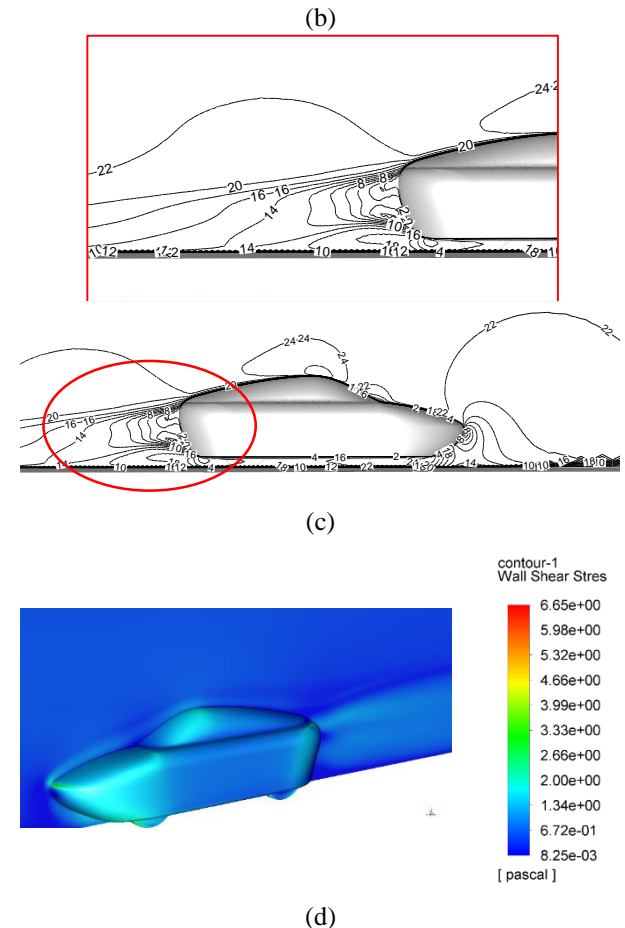
Figure 9. (a) Pressure, (b) Turbulent Kinetic Energy , (c) Velocity Magnitude, and (d) Wall Shear Stress figures at 22.22 m/s
