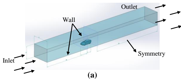
Figure 2. (a) Flow domain design and boundary regions.
