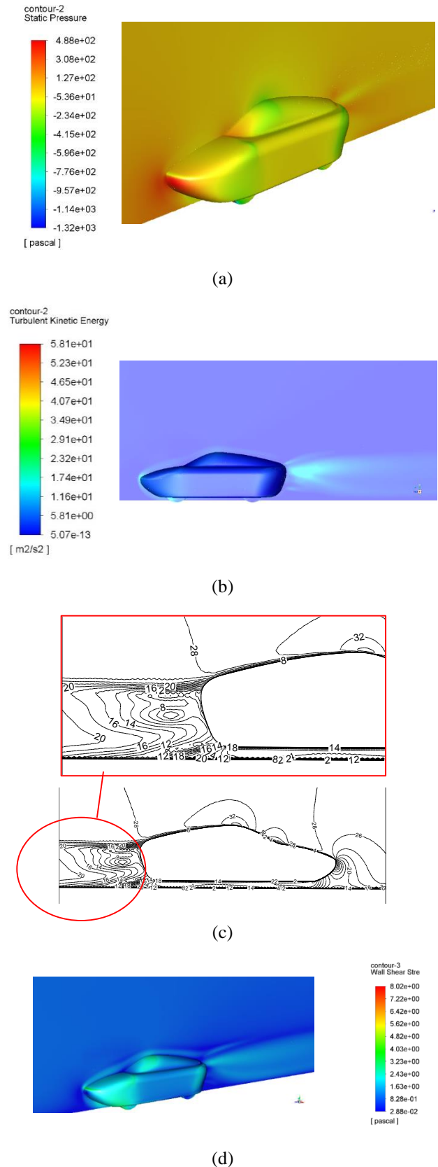
Figure 10. (a) Pressure, (b) Turbulent Kinetic Energy , (c) Velocity Magnitude, and (d) Wall Shear Stress figures at 27.78 m/s
