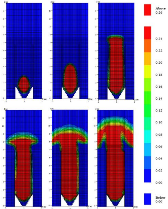
Figure 10. Simulated flame progression. Contours show the mass fraction of the combustion product (kg/kg). Six time intervals are depicted: 0.384 s, 0.428 s, 0.505 s, 0.520 s, 0.531 s, and 0.550 s. Condition set 1. A=2.84 m 2 . P stat = 0.03 bar (3 kPa).) [61]
