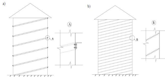
Figure 8. Spiral silo variations: a) spiral bolted; b) spiral welded [49]
