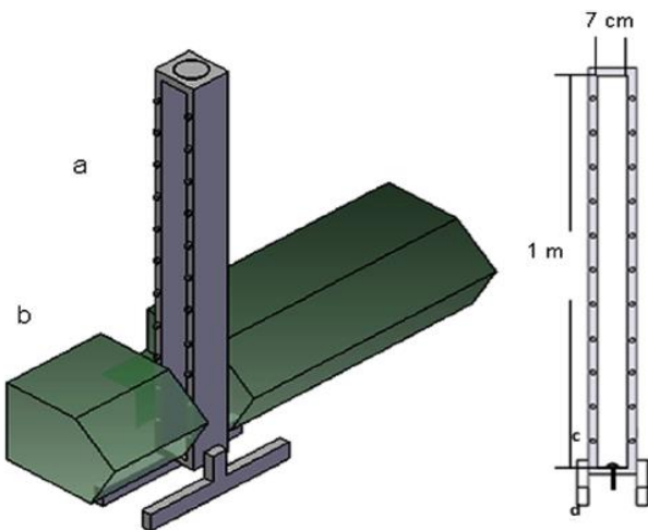
Figure 11. Experimental apparatus designed for analyzing solid material dispersion. a) Dispersion Tube, b) Particle dimension spread analyzer, c) Dispersion Nozzle, d) Gas Inlet) [62].
