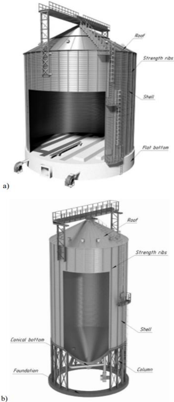
Figure 6. Elevated (conical bottom) and above ground (flat bottom) silos: a) above ground (flat bottom silo), b) elevated (conical bottom silo) [49]
