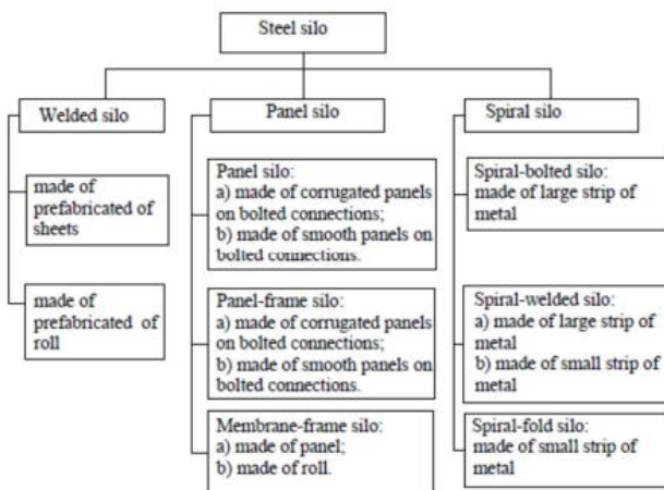
Figure 4. Classification of metal silos
