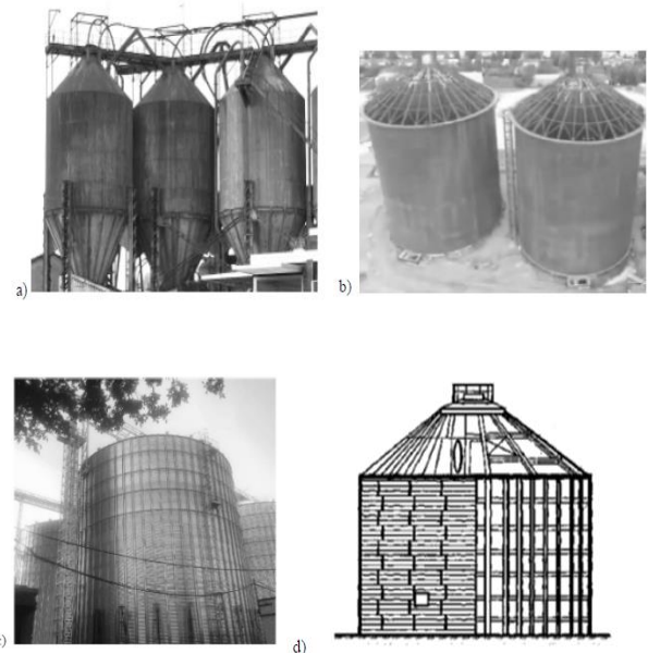
Figure 7. Different types of metal silos: a, b) welded silos; c) panel type; d) panel frame type) [49]
