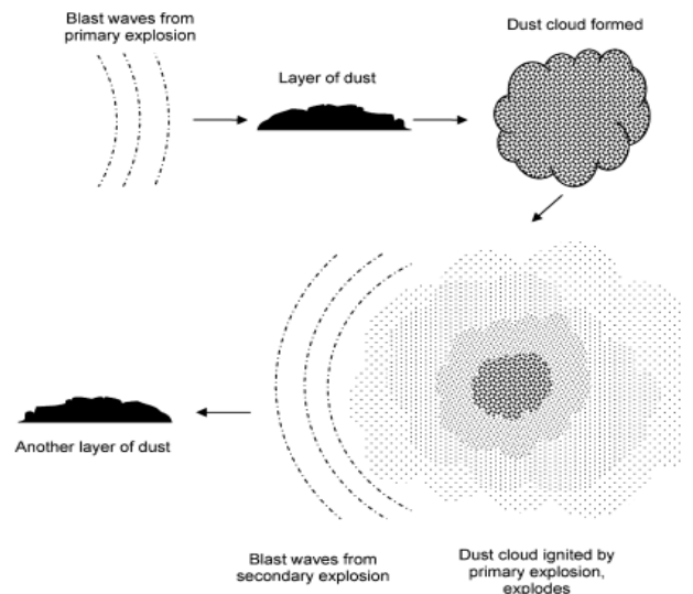
Figure 3. Chain reaction in dust explosion)
